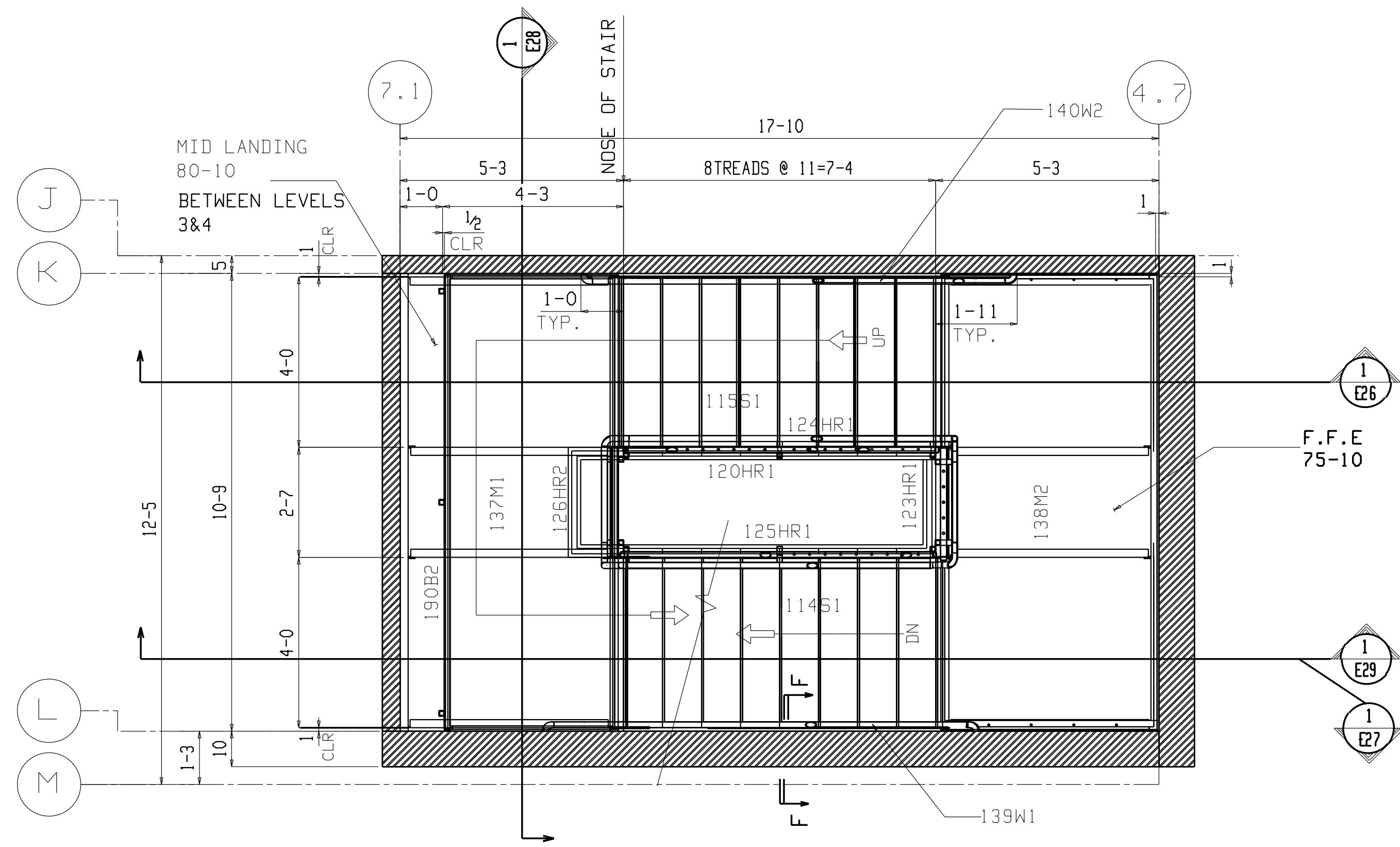
3rd FLOOR STAIR #6 PLAN OF AREA-B Elevation: 75-10 (U.N.O)
