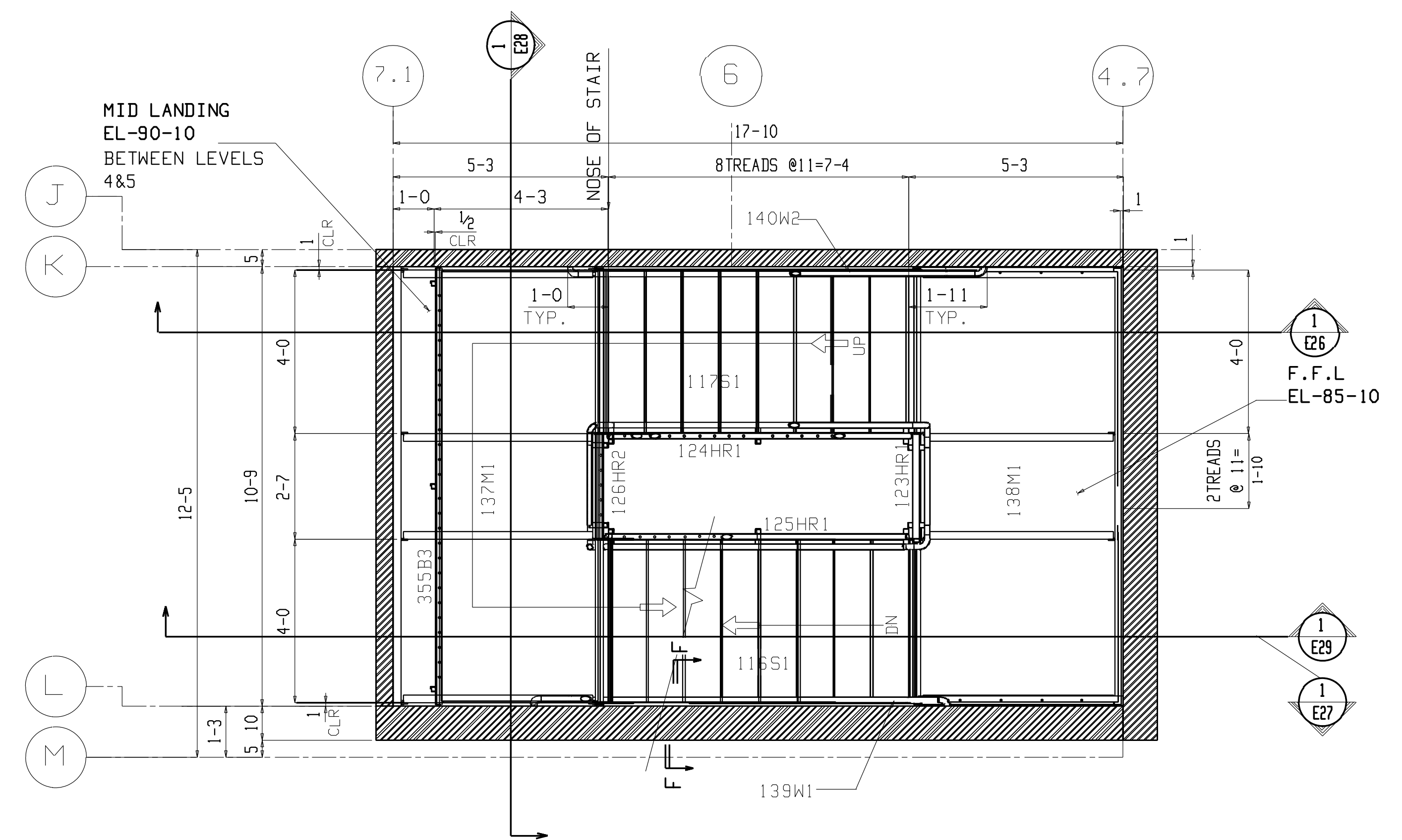
4th FLOOR STAIR #6 PLAN OF AREA-B Elevation: 85-10 (U.N.O)
